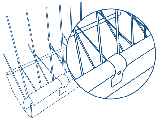
Proprietary (intergrated) mounting tab that folds over any spout lip
