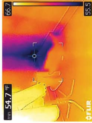
Area box with Cold Spot demonstrates air infiltration
